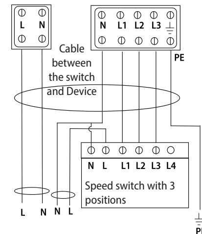
Figure 4 – Connecting the power cable to a Device equipped with an external fan speed switch.
